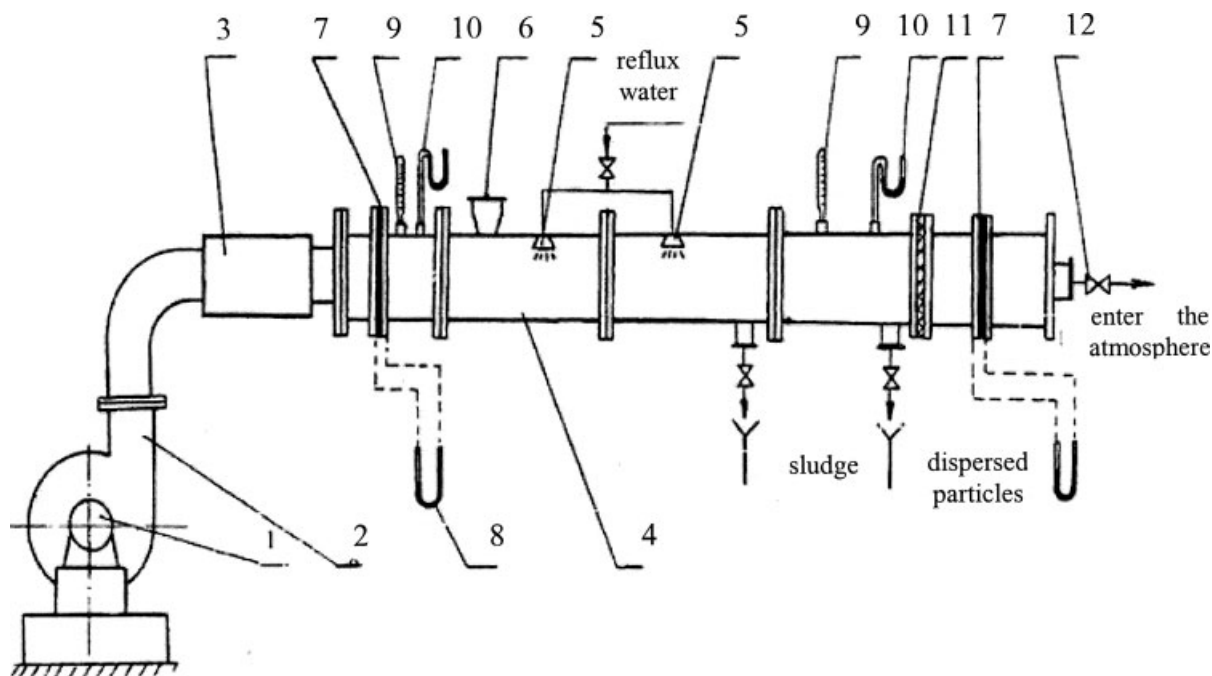
Figure 1 Flow diagram of the experimental unit: 1 – electric motor; 2 – ventilator (fan); 3 – electric heater; 4 – rotation chamber (cell); 5 – sprayers; 6 – bunker; 7 – diaphragm; 8 – pressure-gauge; 9 – thermometer; 10 – manometer; 11 – filter; 12 – valve.
