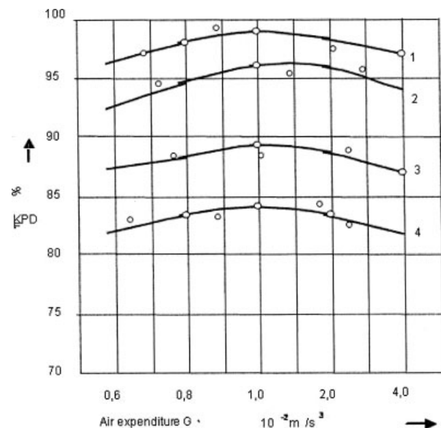
Figure 4 Dependence of the device efficiency on air expenditure at constant water expenditure ( Q = 8.5 \times 10^{-3} \text{ m}^3/\text{s} ) for different profiles of the rotator blades. 1 – parabolic; 2 – hyperbolic; 3 – sine wave; 4 – direct.
