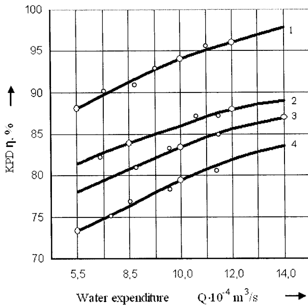
Figure 3 Dependence of the device efficiency on water expenditure at constant air expenditure ( G = 40 \times 10^{-3} \text{ m}^3/\text{s} ) for different profiles of the rotator blades. 1 – parabolic; 2 – hyperbolic; 3 – sine wave; 4 – direct.
