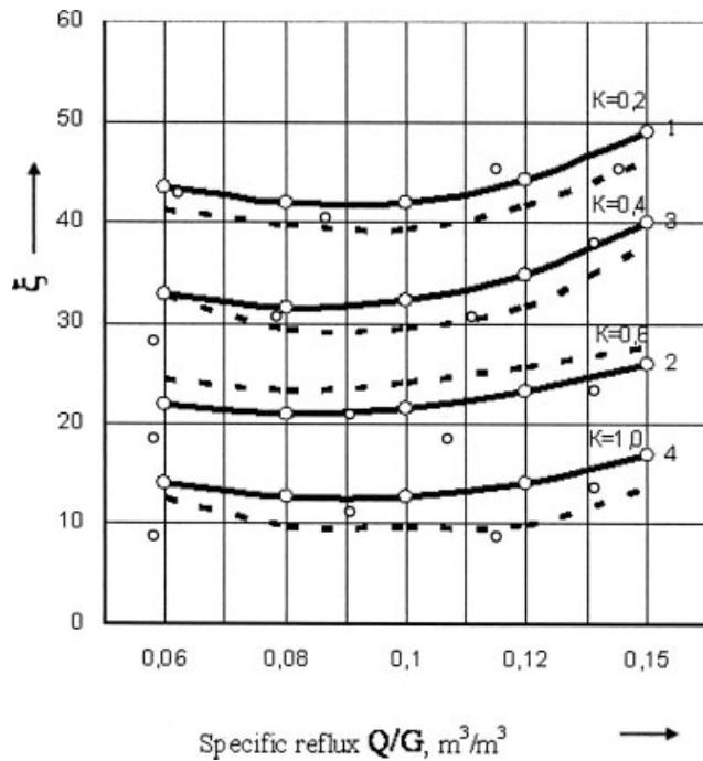
Figure 5 \xi dependence on specific reflux of the device with different values of curling efficiency.
